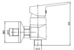
Art. No. A 807U 0000 Shower Mixer Art. No. A 817U 0000 Shower Mixer with handshower, wall support and flexible hose 150 cm
